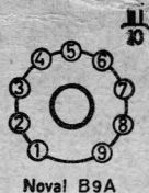
Noval B9A
